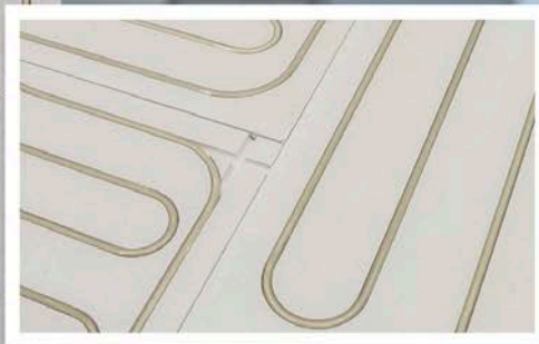
Wall heating in dry method
